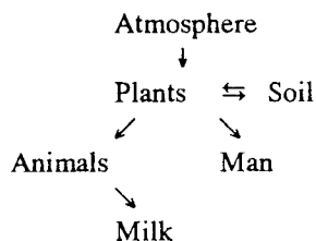
Figure 1. Main Terrestrial Pathways in the Food Chain for Radiostrontium (5)
