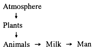
Figure 2. Main Terrestrial Pathway in the Food Chain for Barium 140 (5)
